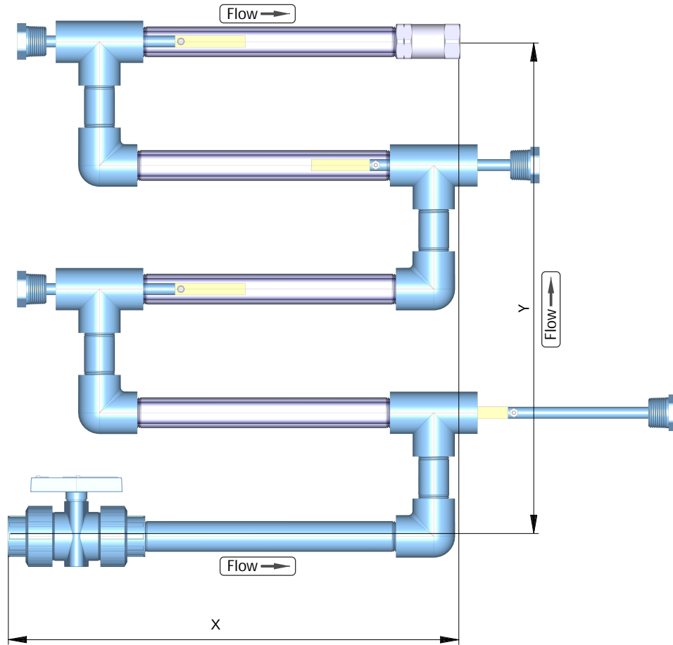
Approximate Dimensions (inches) for 1" NPT pipe, 0.60" thread engagement
